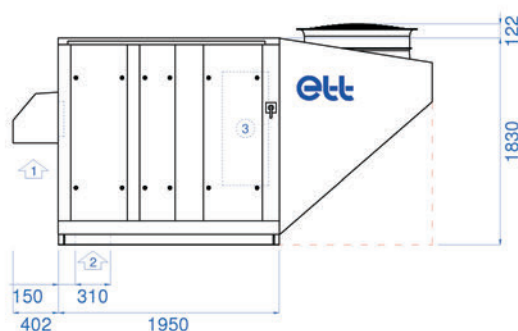
Side SUPPLY AIR
