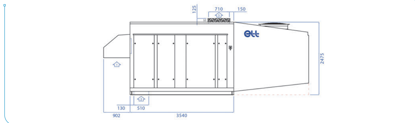
Front view:
