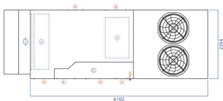
Supply air side view :
