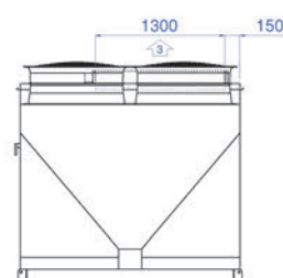
Supply air side view :
