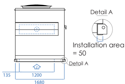
Return air side view:
