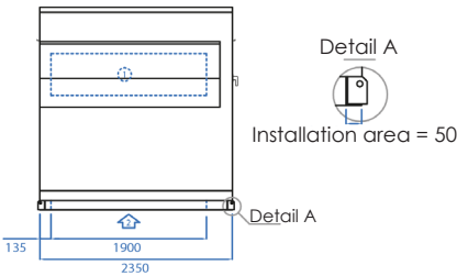
Return air side view:
