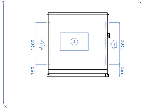
Exhaust air side view:
