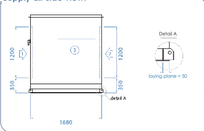
Supply air side view:
