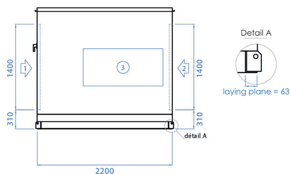
Supply air side view:
