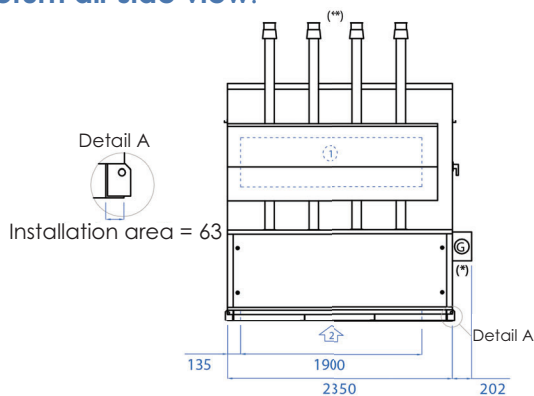
Return air side view:
